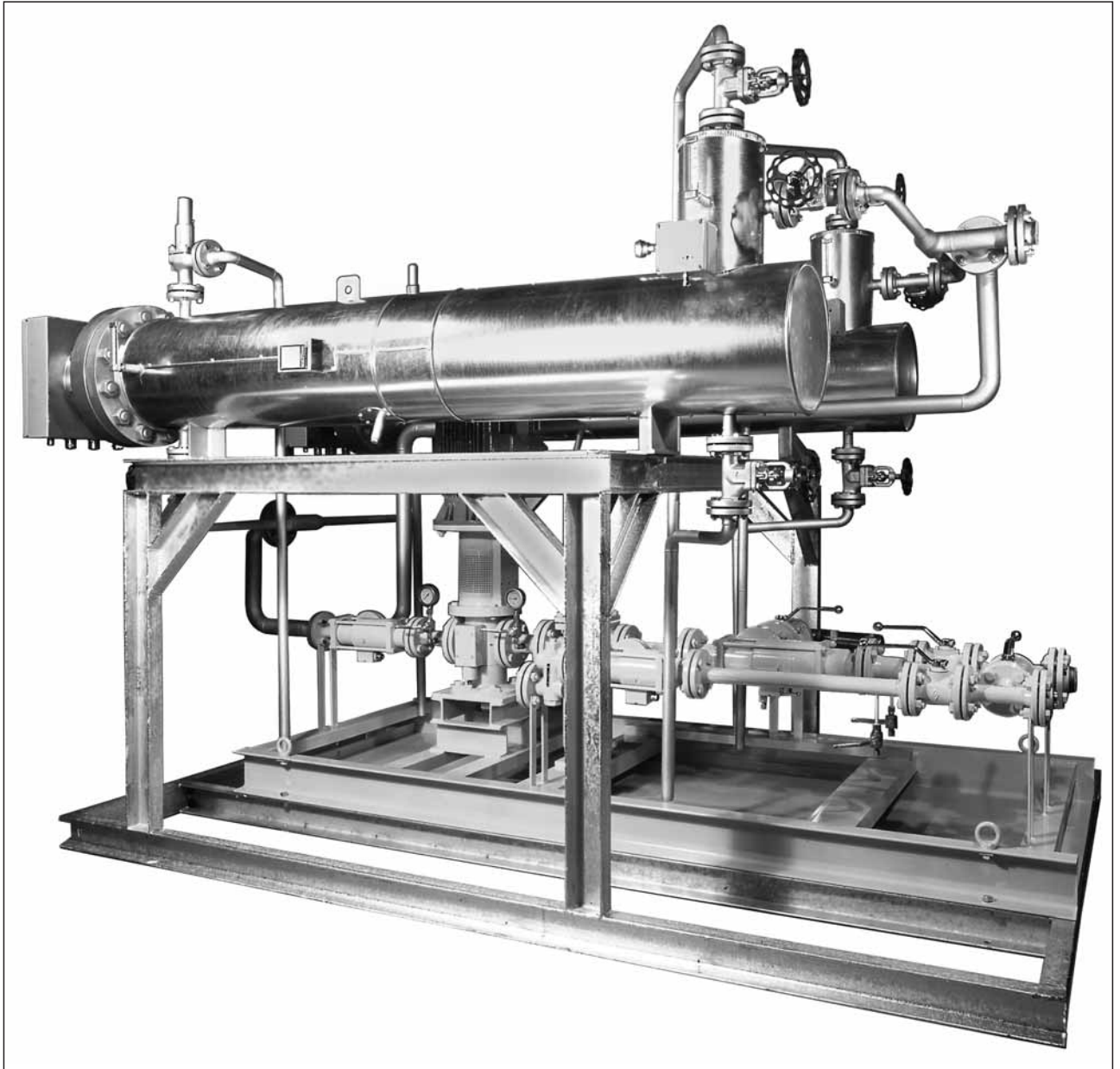
Electric heavy oil pre-heater, complete with pump, fittings and piping, mounted on steel frame, ready to connect version. Capacity 2 x 140 kW.
