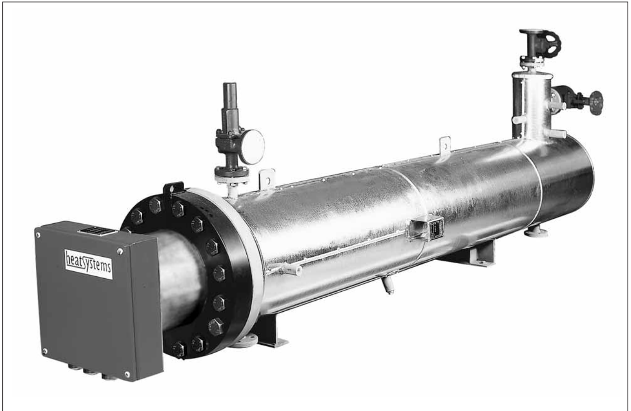
Electric heavy oil pre-heater. Capacity 180 kW.
